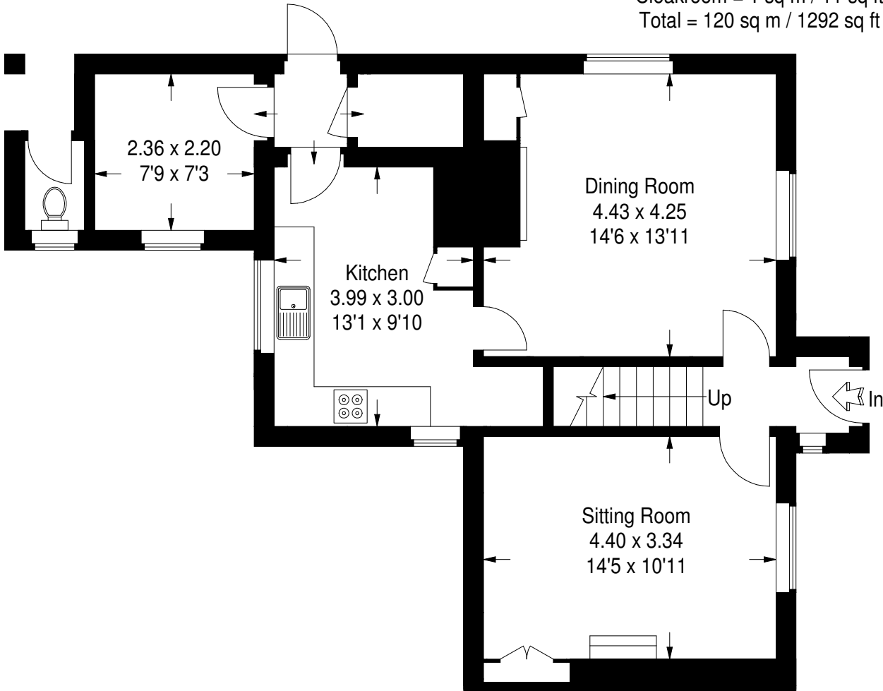
Ground Floor
